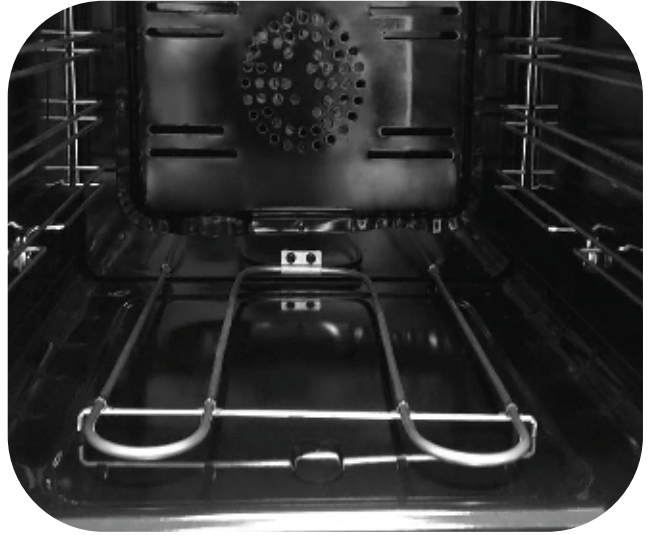
Foldable Element
